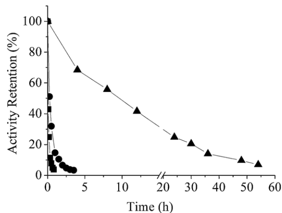
Fig. 2. Thermal stability at 55 °C of chitosan-immobilized \beta -D-galactosidase in the presence of 400 g L -1 lactose solutions (▲), 50 g L -1 lactose solutions (●), and activity buffer (■).
