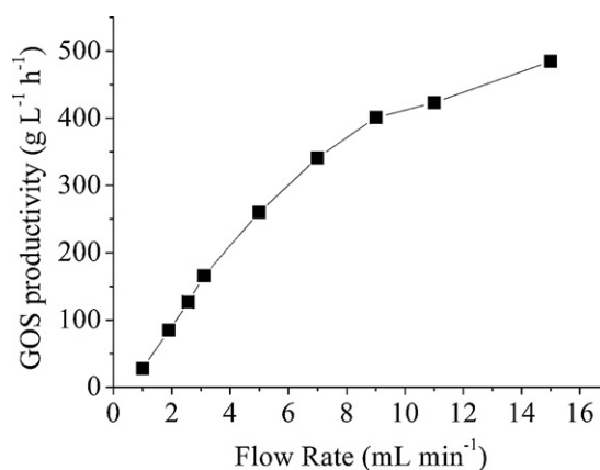
Fig. 6. Effect of flow rate on GOS productivity. Experiments were performed using 400 g L -1 buffered lactose solution, pH 7 at 37 °C.
