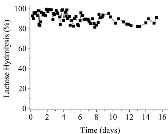
Fig. 7. Operational stability of the PBR filled with chitosan-immobilized \beta -D-galactosidase, operated continuously using 50 g L -1 buffered lactose solution, pH 7 at 37 °C and flow rate of 2.6 mL min -1 .
