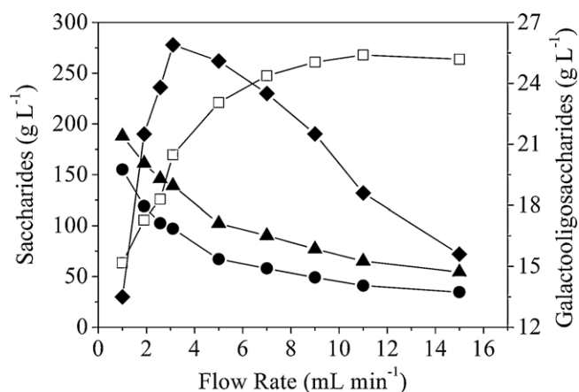
Fig. 5. Effect of flow rate on GOS synthesis by chitosan-immobilized \beta -D-galactosidase, using 400 g L -1 buffered lactose solution, pH 7 at 37 °C. D-Glucose (▲), D-galactose (●), lactose (□), and galactooligosaccharides (◆).
